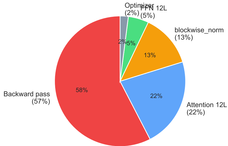
Training Step Breakdown (27.4ms, N=200, d=320, 6L+6L)
