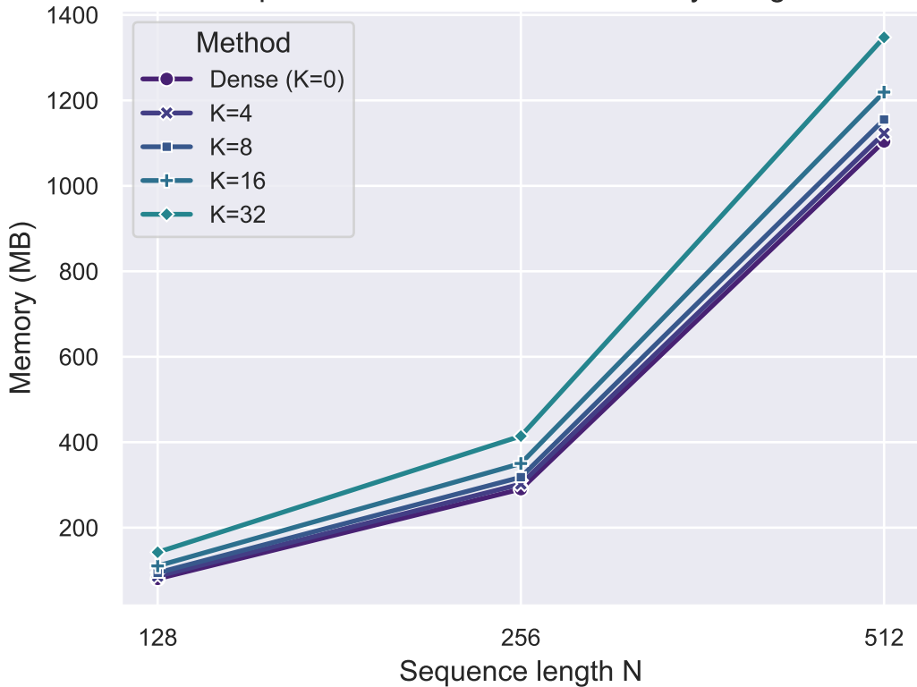
Sparse Attention — Peak Memory Usage
