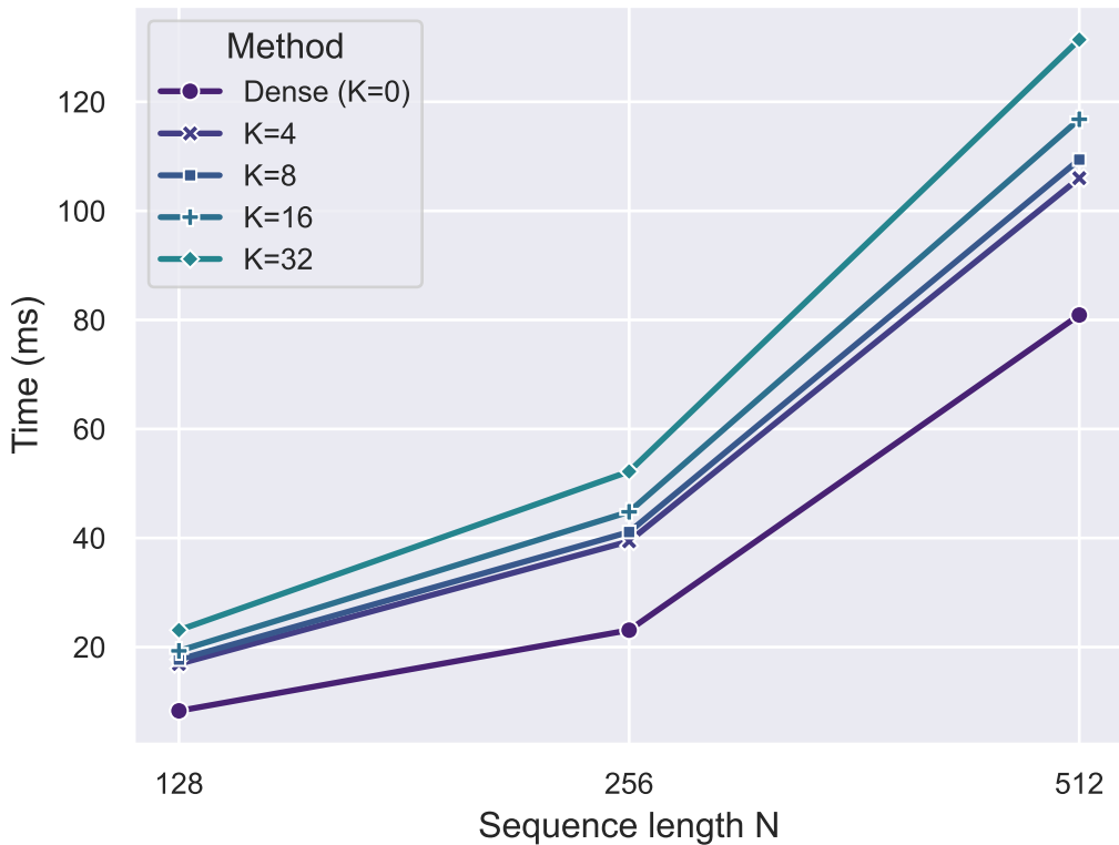
Sparse Attention — Forward Speed
