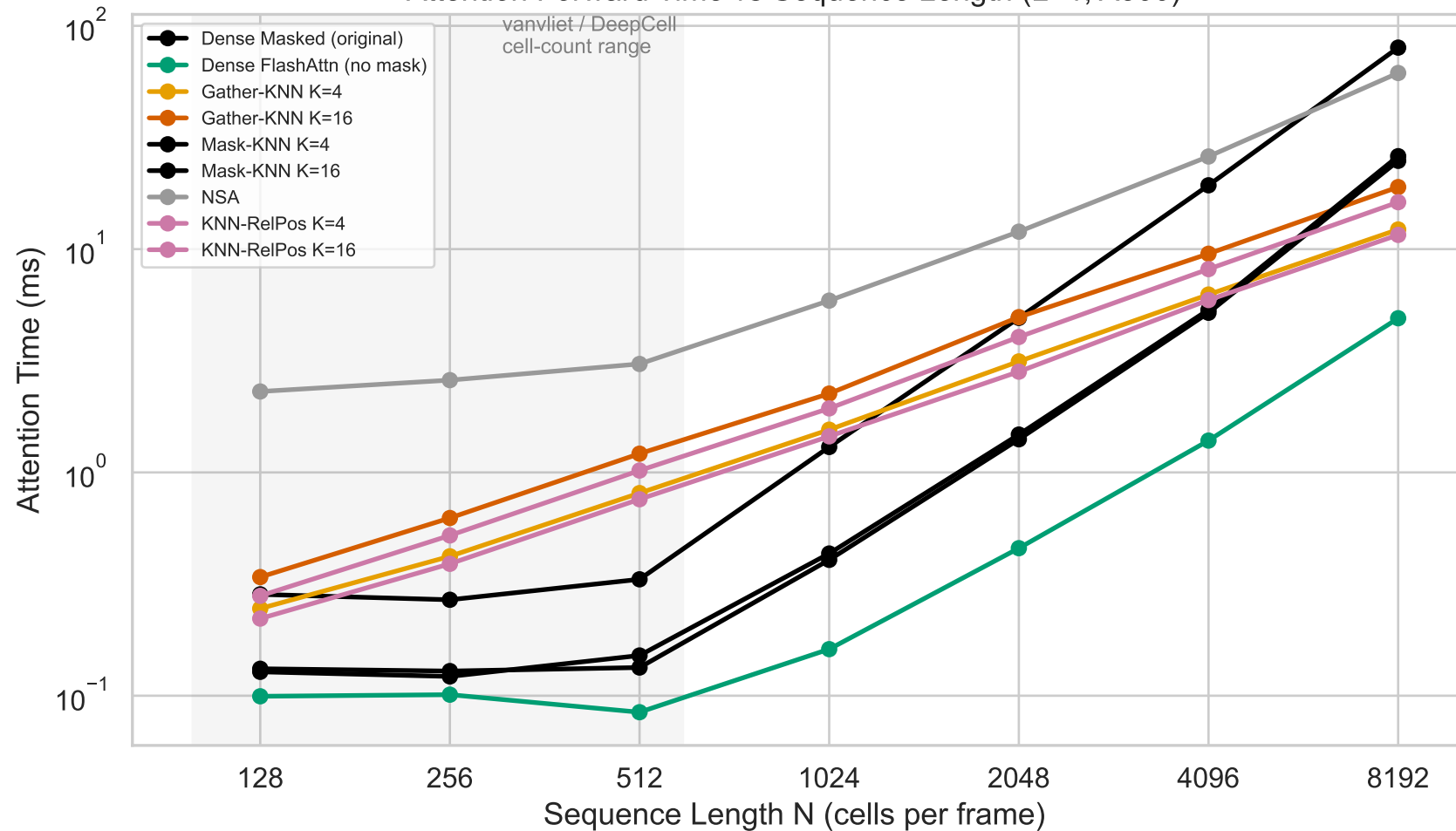
Attention Forward Time vs Sequence Length (L=1, A500)
