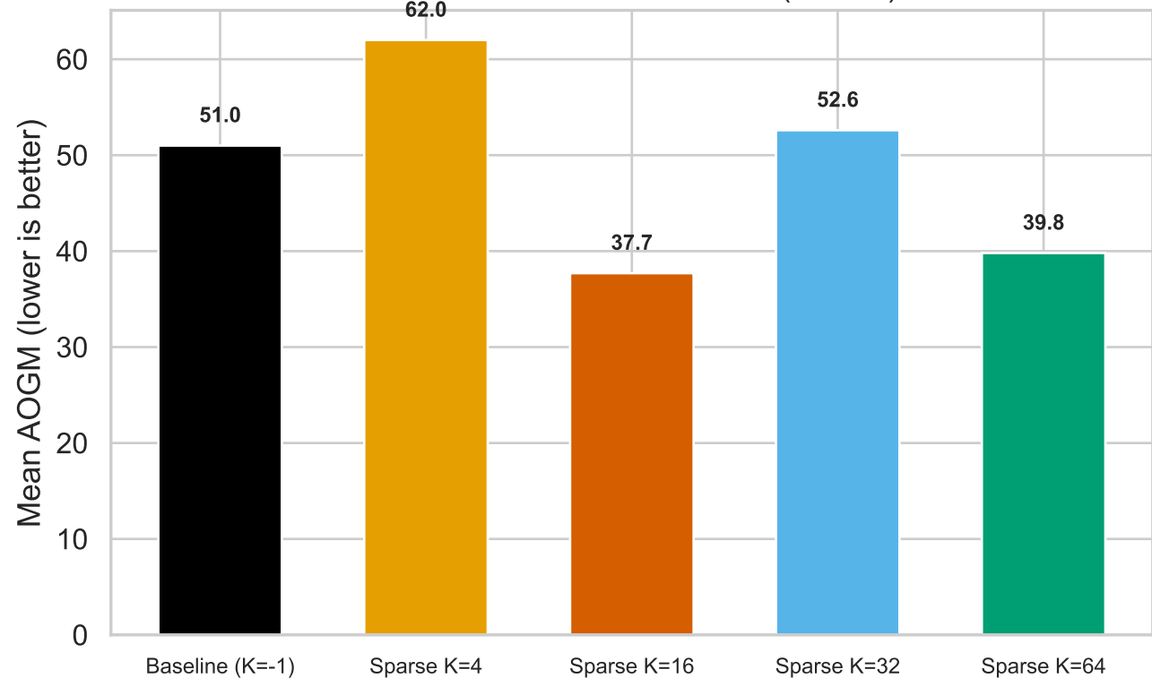
Detection + Association Error (AOGM)
