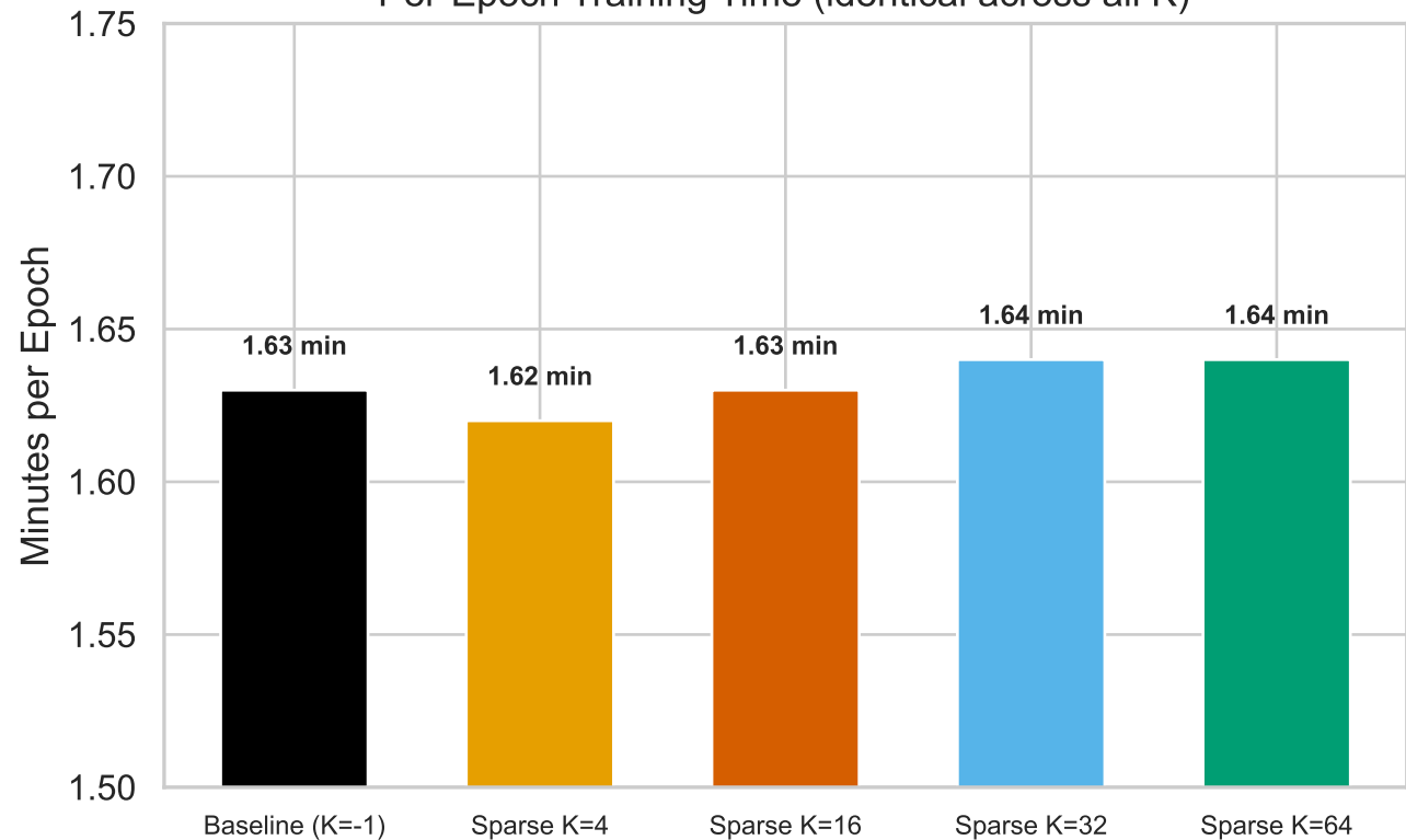
Per-Epoch Training Time (identical across all K)
