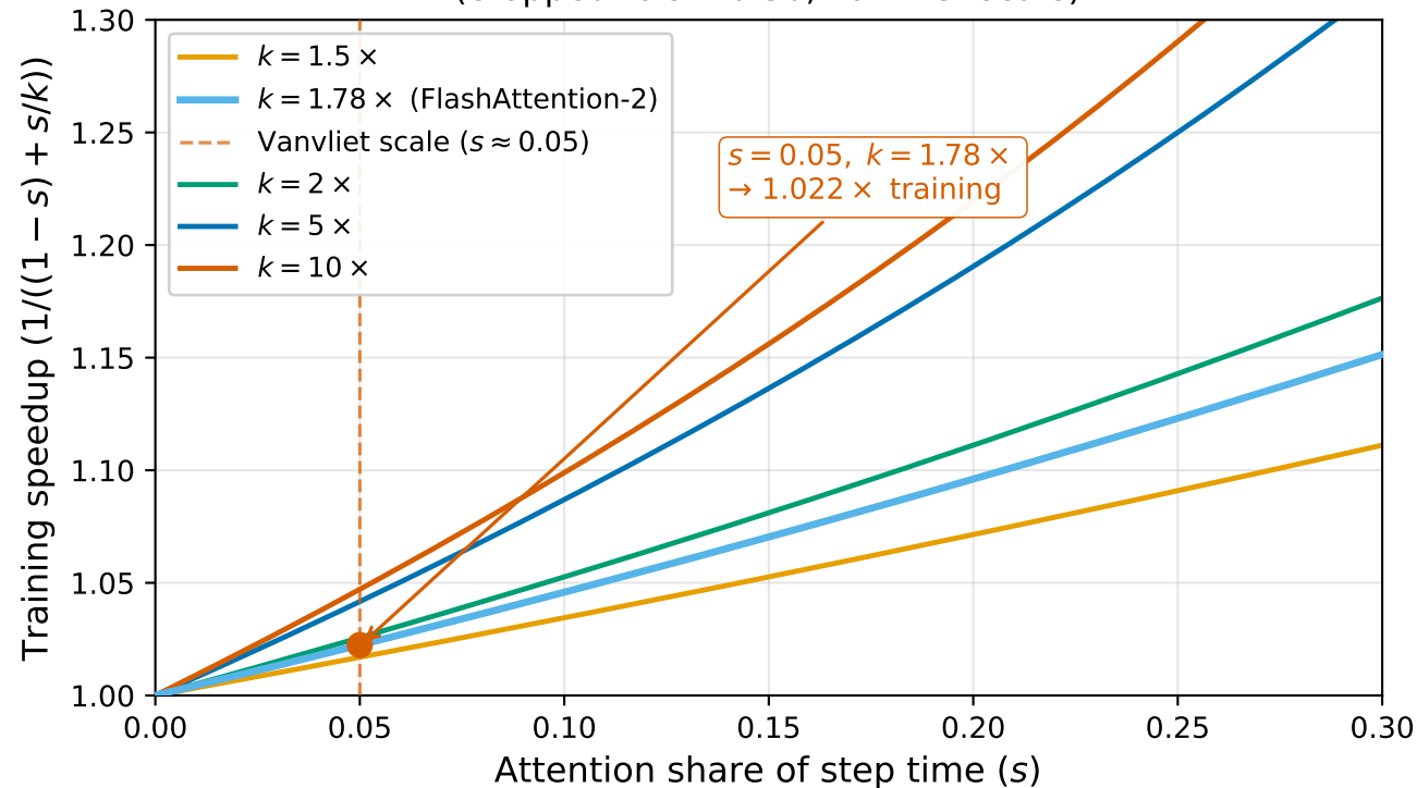
Amdahl's Law: Training Speedup vs. Attention Share (cropped to s \leq 0.30 , vanvliet scale)
