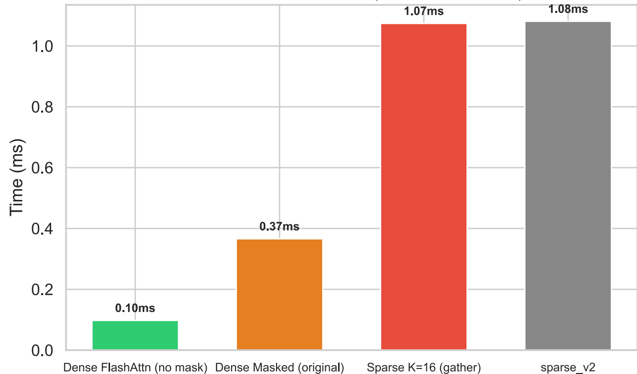
Attention Time at N=256 (Real Dataset Size)
