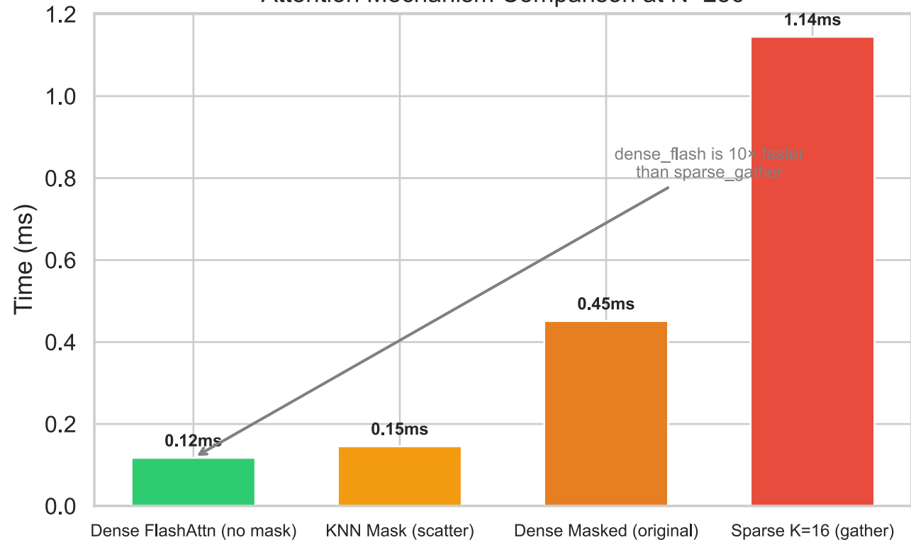
Attention Mechanism Comparison at N=256
