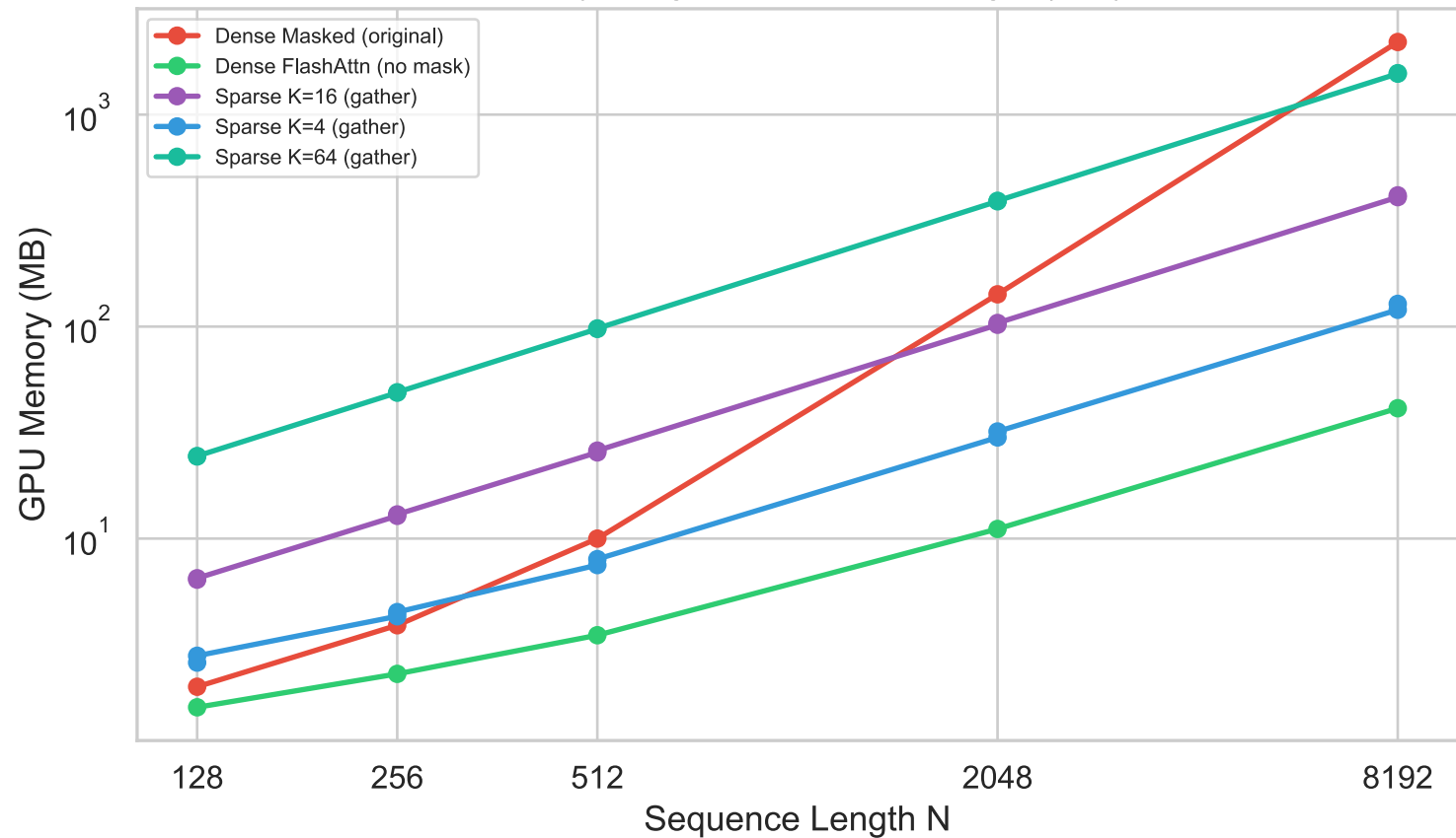
Memory Usage vs Sequence Length (L=1)
