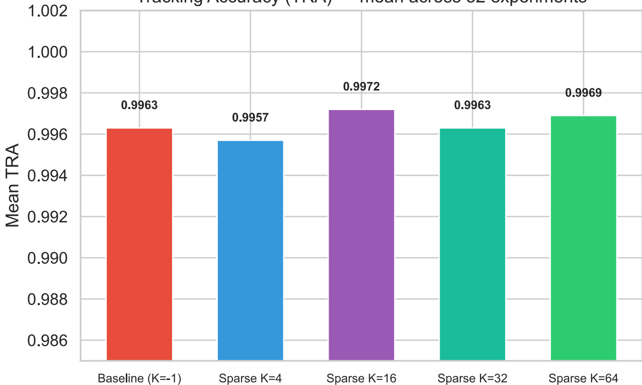
Tracking Accuracy (TRA) — mean across 32 experiments
