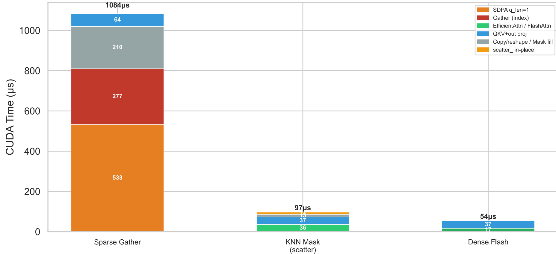
Forward Pass Breakdown at N=256 — Per-Operation (torch.profiler)
