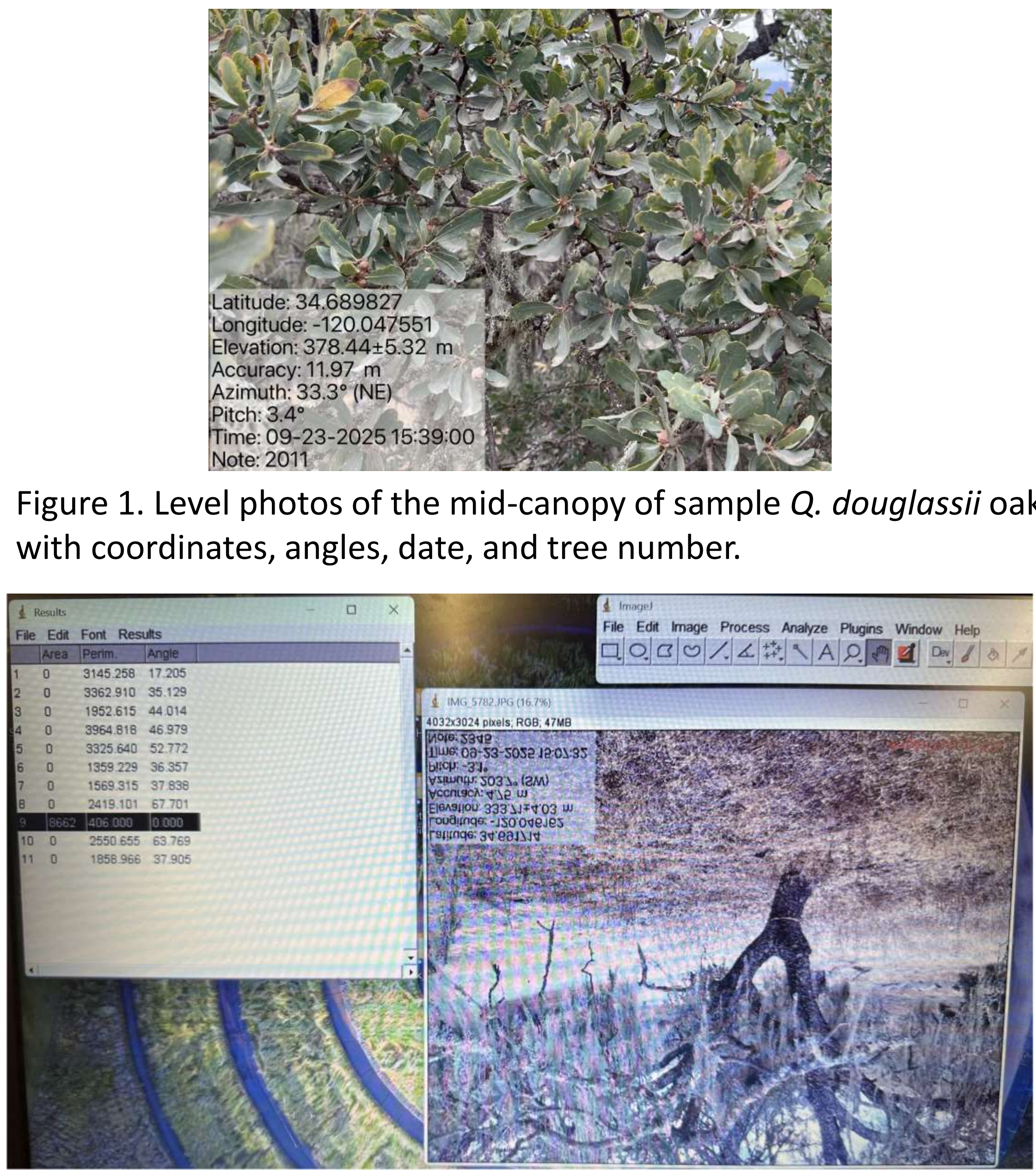
Figure 1. Level photos of the mid-canopy of sample Q. douglassii oak with coordinates, angles, date, and tree number. Figure 2. Oak image (flipped upside down) on ImageJ with ten leaf angle measurements taken (top left).
