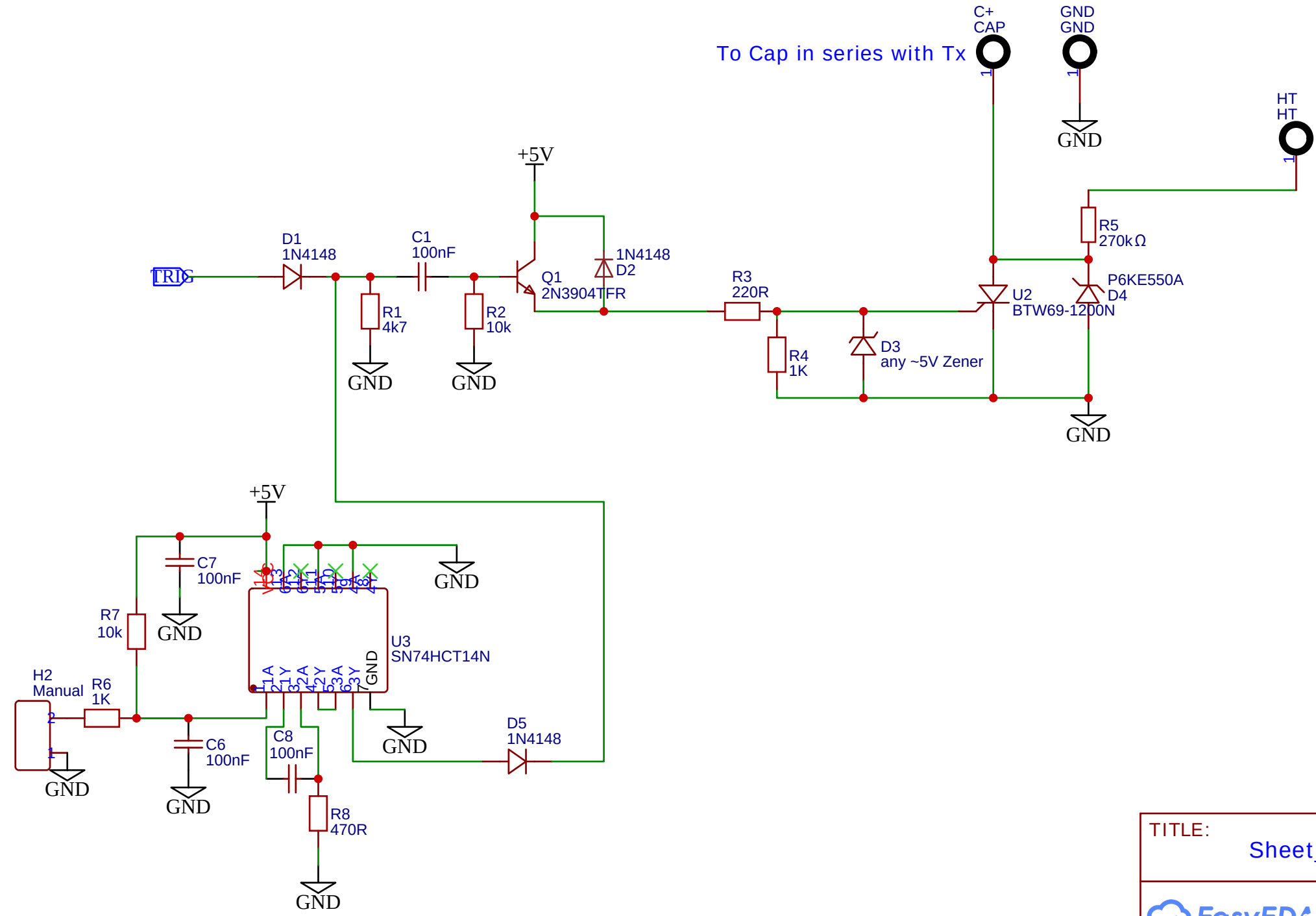
Trigger Circuit
