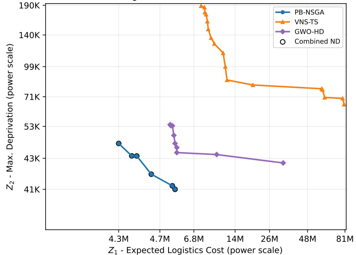
(b) CV-Large: PB-NSGA vs VNS-TS vs GWO-HD
