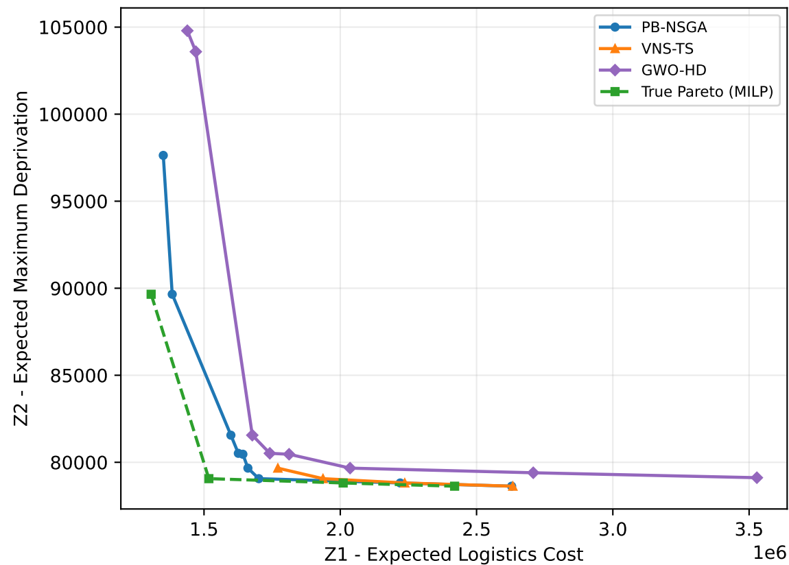
(a) CV-Small: PB-NSGA vs VNS-TS vs GWO-HD vs True Pareto
