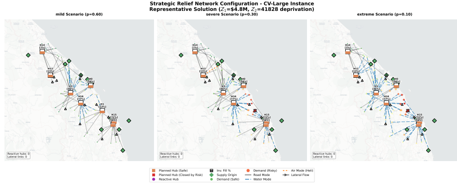
Fig. 3: CV-Large knee-point relief network ( Z_1=\$4.8\text{M} , Z_2=41,828 ) across three flood scenarios. Hub colours and line styles as per legend.
