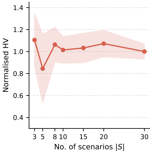
Pareto front quality (HV)
