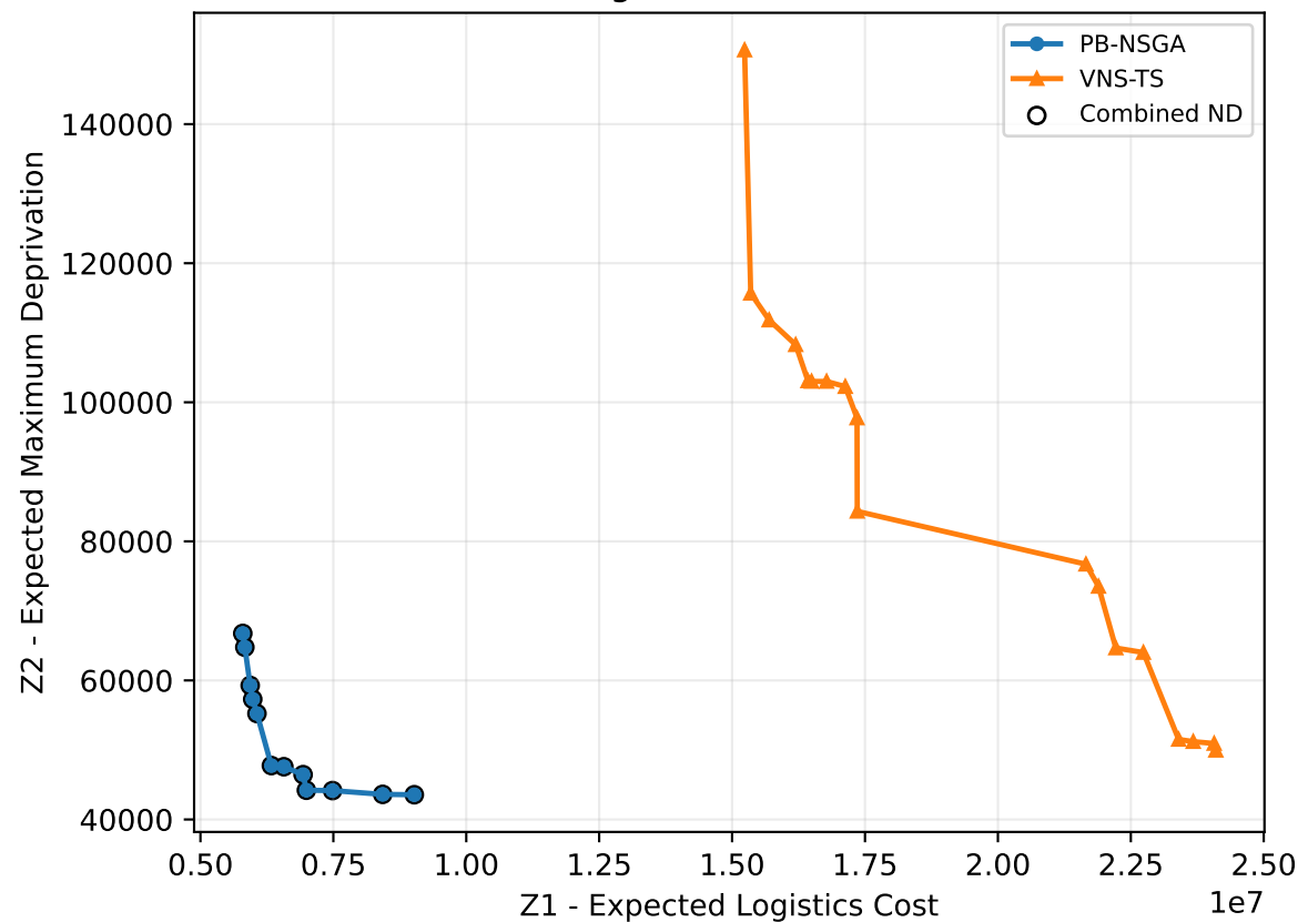
(b) CV-Large: PB-NSGA vs VNS-TS
