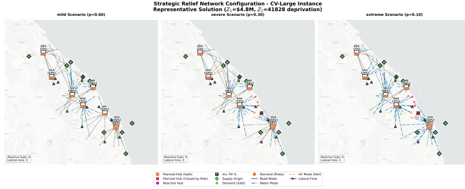
Fig. 3: CV-Large knee-point relief network ( Z_1 =$4.8M, Z_2 =41,828) across three flood scenarios. Hub colours and line styles as per legend.
