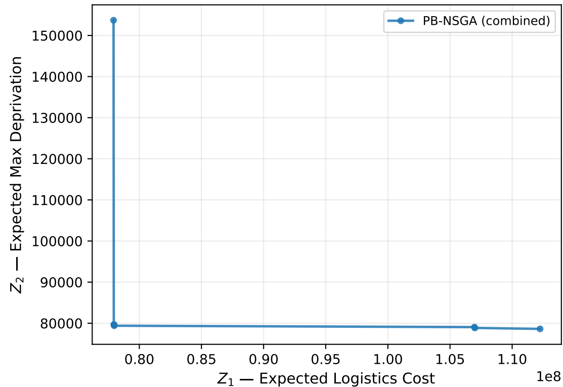
Pareto Front — Cv Small (3 seeds)
