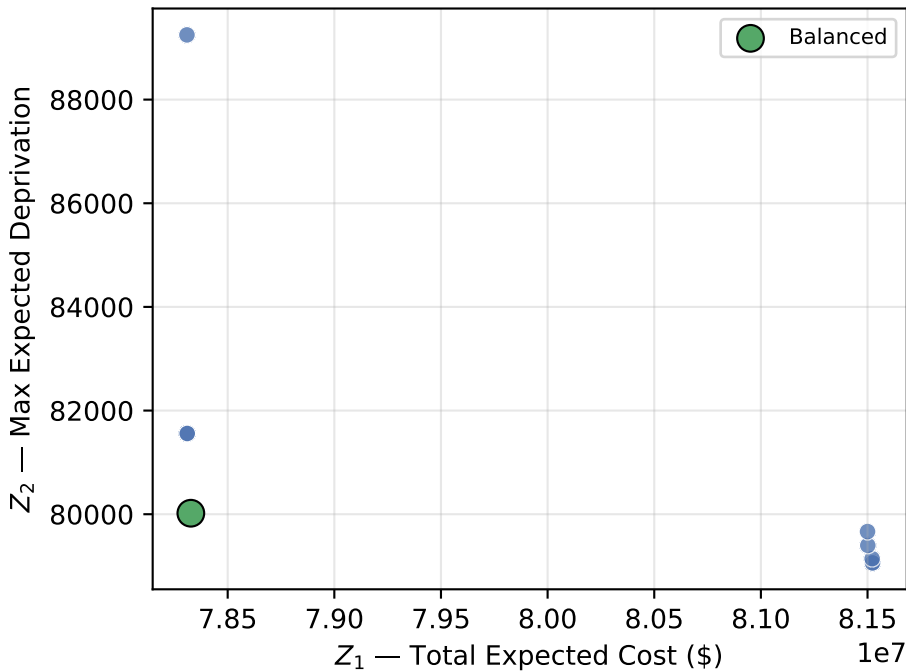
PB-NSGA-II: Pareto Front (CV-Small)
