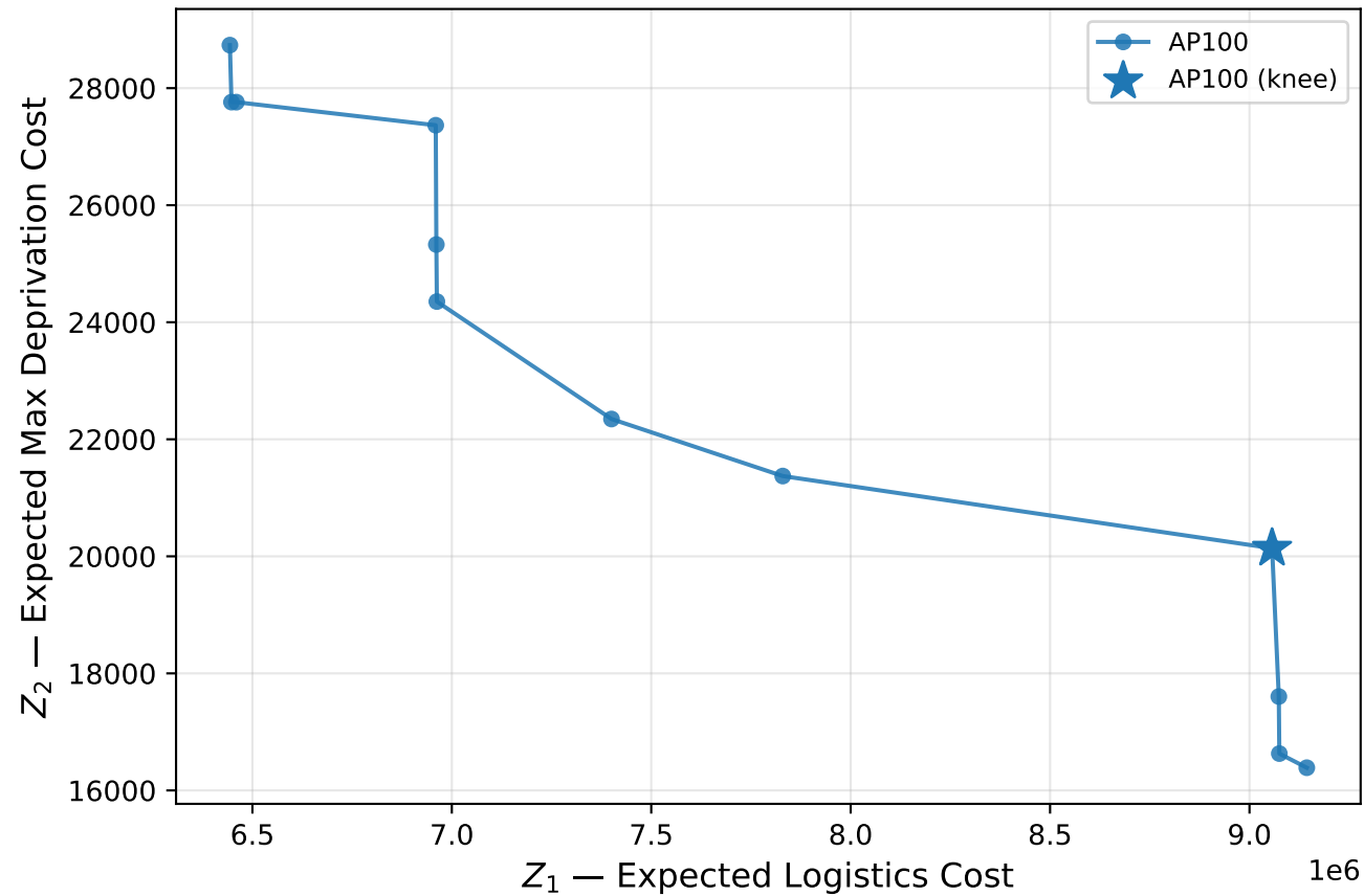
Pareto Front — AP100 Benchmark
