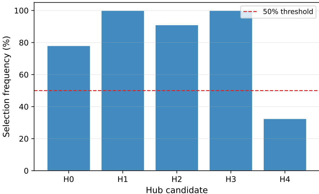
Hub Selection Frequency — Cv Small
