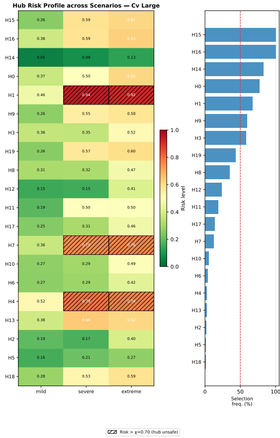
Fig. 4. Geophysical risk profile and safety filter ( r_{ks} \leq \chi = 0.70 ) status of candidate hubs across flood scenarios, explaining dynamic recourse behavior.
