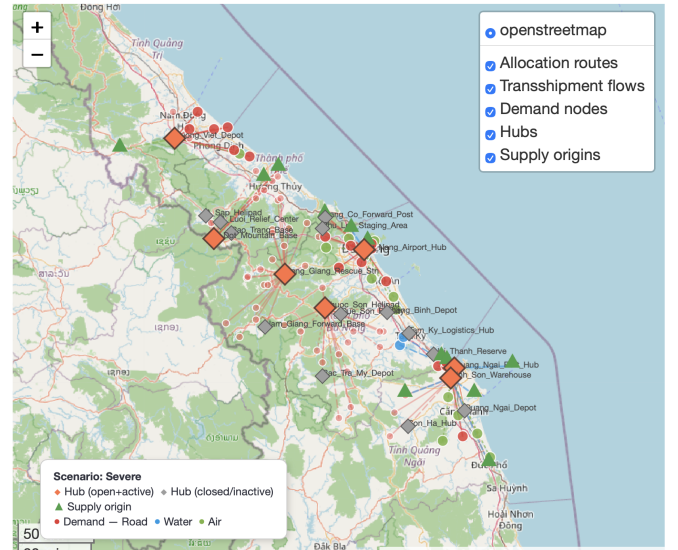
Fig. 2. Geospatial solution map rendered within the DSS for a compromise solution ( Z_1 = \$4.8M, Z_2 = 41,828 ), demonstrating structural hub filtering and multi-modal routing adaptation under Severe flood scenarios.
