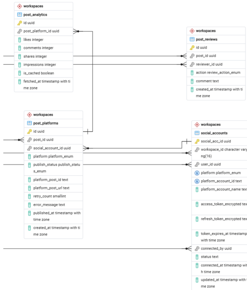
Figure. Review, Social Media Publishing, and Post Analytics ERD
