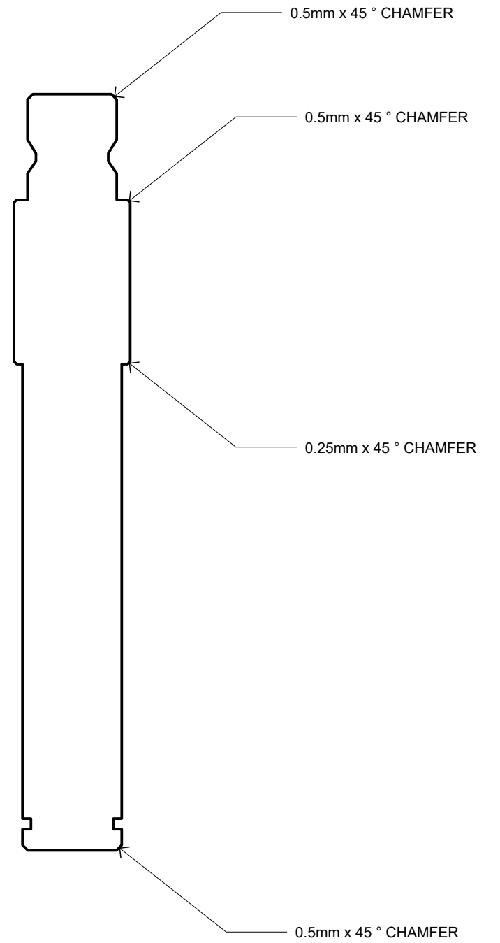
CHAMFERS
