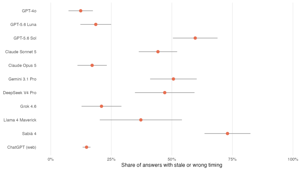
Figure 3: Each point is the share of a model’s answers the coder flagged for stale timing: the election treated as future or undated, registered candidates described as unconfirmed, or outdated facts; whiskers are 95% intervals across prompts. Full profiles, specific-candidate wording.
