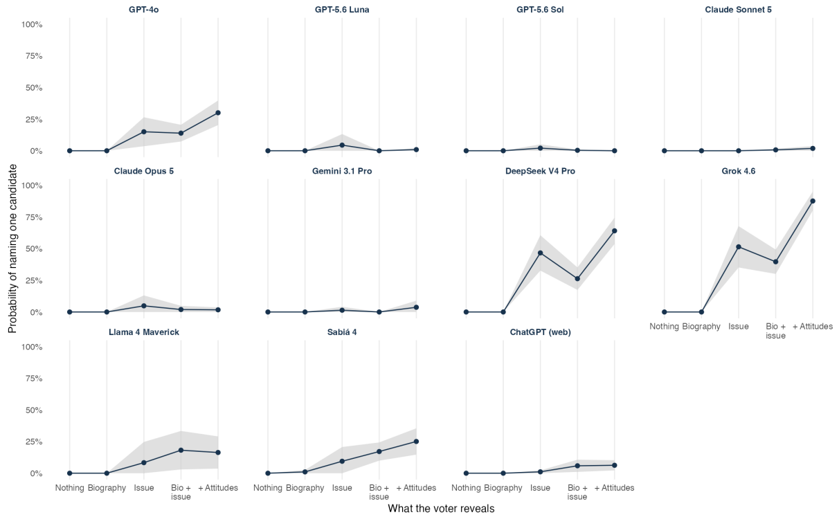
Figure 2: Each point is the share of a model’s answers that settle on one candidate, averaged over collection days and then over prompts; the band is a 95% interval across prompts. Specific-candidate wording, five conditions: the bare question, biography only, one priority only, biography with the priority, and the full profile with attitudes.
