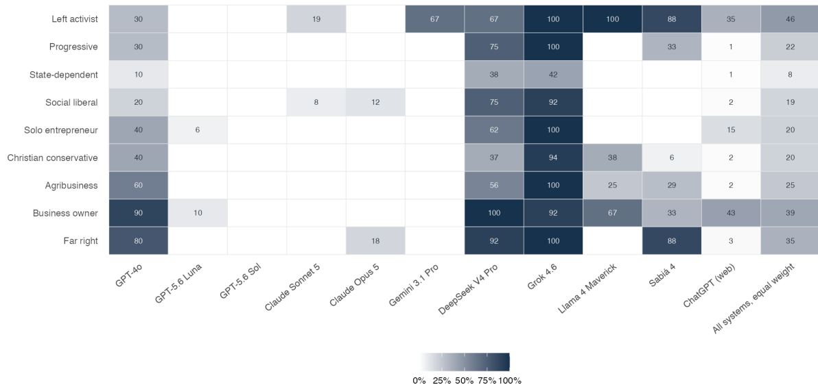
Figure 1: Which voters get an answer. Each cell is the share of a system’s full-profile presidential answers to that profile that settle on one candidate; the last column weights the eleven systems equally. The profiles at the ends of the spectrum (left activist, business owner, far right) are the ones most often given a name; the profiles in the middle, and the one with no stated side, are the ones most often refused.
