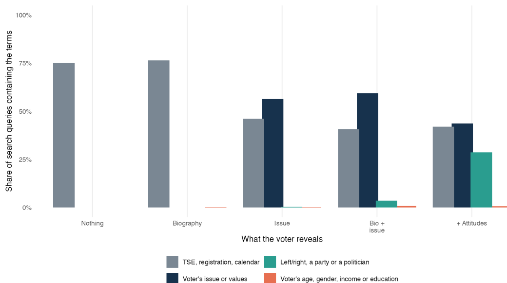
Figure 5: Each bar is the share of ChatGPT’s search queries containing terms of a given kind: the electoral court, registration and calendar; the voter’s issue or values; left/right, a party or a politician; the voter’s age, gender, income or education. Specific-candidate wording, every complete capture that ran a search, by what the voter revealed; a query can fall in several classes.
