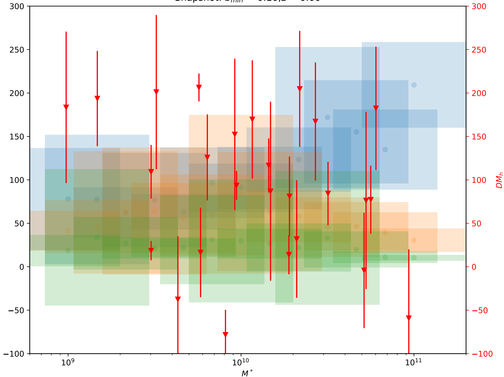
Snapshot: b_{min} = 0.10, z = 0.00
