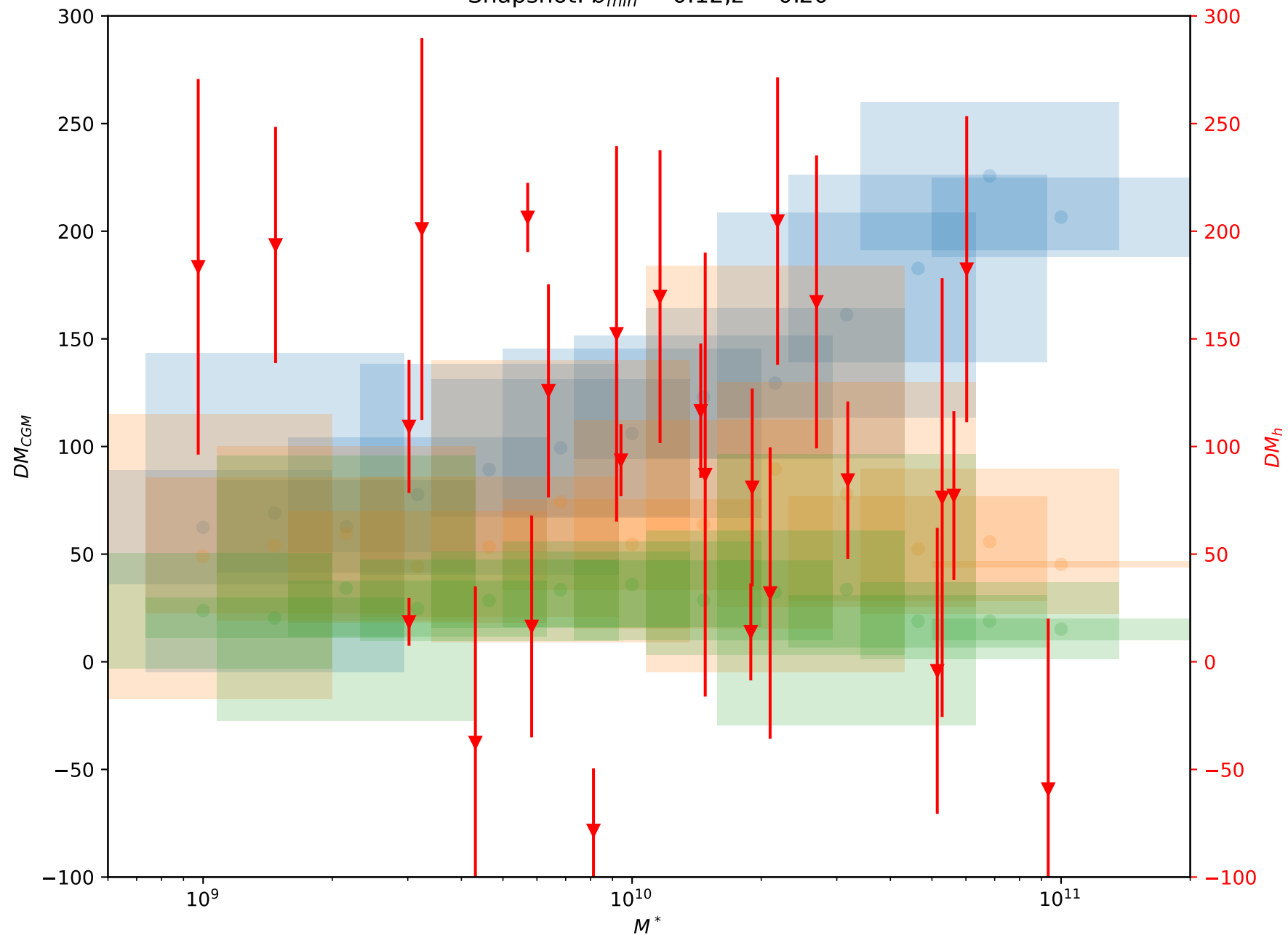
Snapshot: b_{min} = 0.12, z = 0.20
