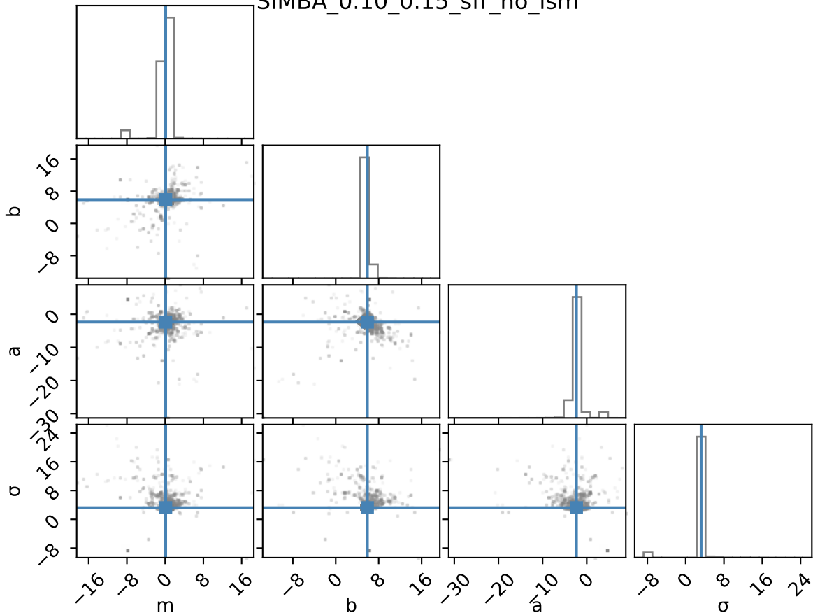
SIMBA_0.10_0.15_sfr_no_ism
