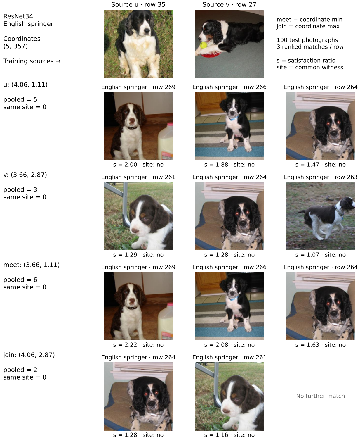
Figure 13: Imagenette springer queries for ResNet34 on coordinates (5, 357). The top row shows the training sources. Subsequent rows show source queries, their meet, and their join, followed by ranked test matches. Here s is the graded satisfaction ratio. The join has two matches; the third position is explicitly empty. None of the pooled matches has a common-site witness.
