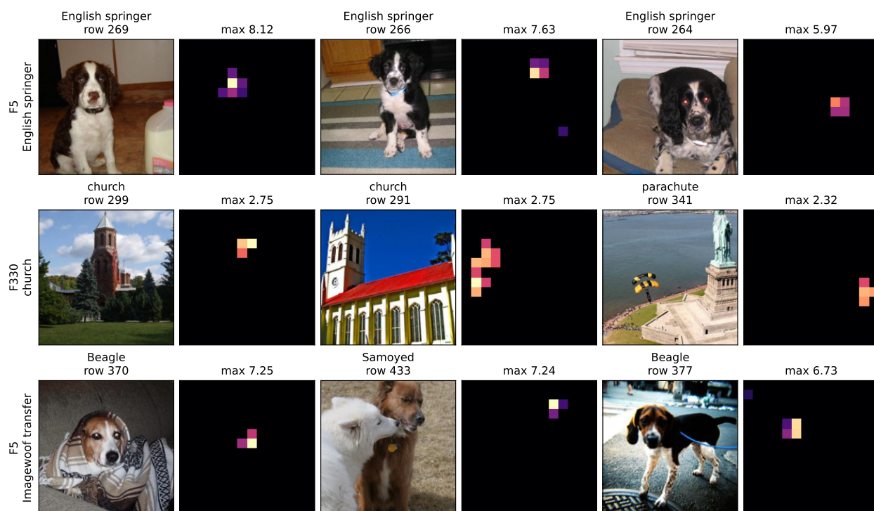
Figure 7: ResNet34 sparse coordinates on Imagenette and Imagewoof. The first two rows show the strongest Imagenette test responses for training-selected springer and church coordinates. The last row applies the springer coordinate to Imagewoof without retraining. Each photograph is followed by its site-code map, with a common color scale within the row. Actual labels, stored dataset rows, and maxima are displayed.
