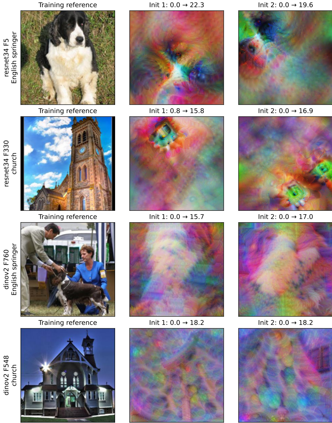
Figure 9: Training reference photographs and two optimized stimuli per coordinate. Titles report actual max-pooled sparse codes before and after optimization, evaluated without jitter. The photographs initialize neither run: optimization starts from random Fourier parameters. Textures or shapes in these images suggest hypotheses, but cannot alone identify semantic feature meanings or a downstream computation.
