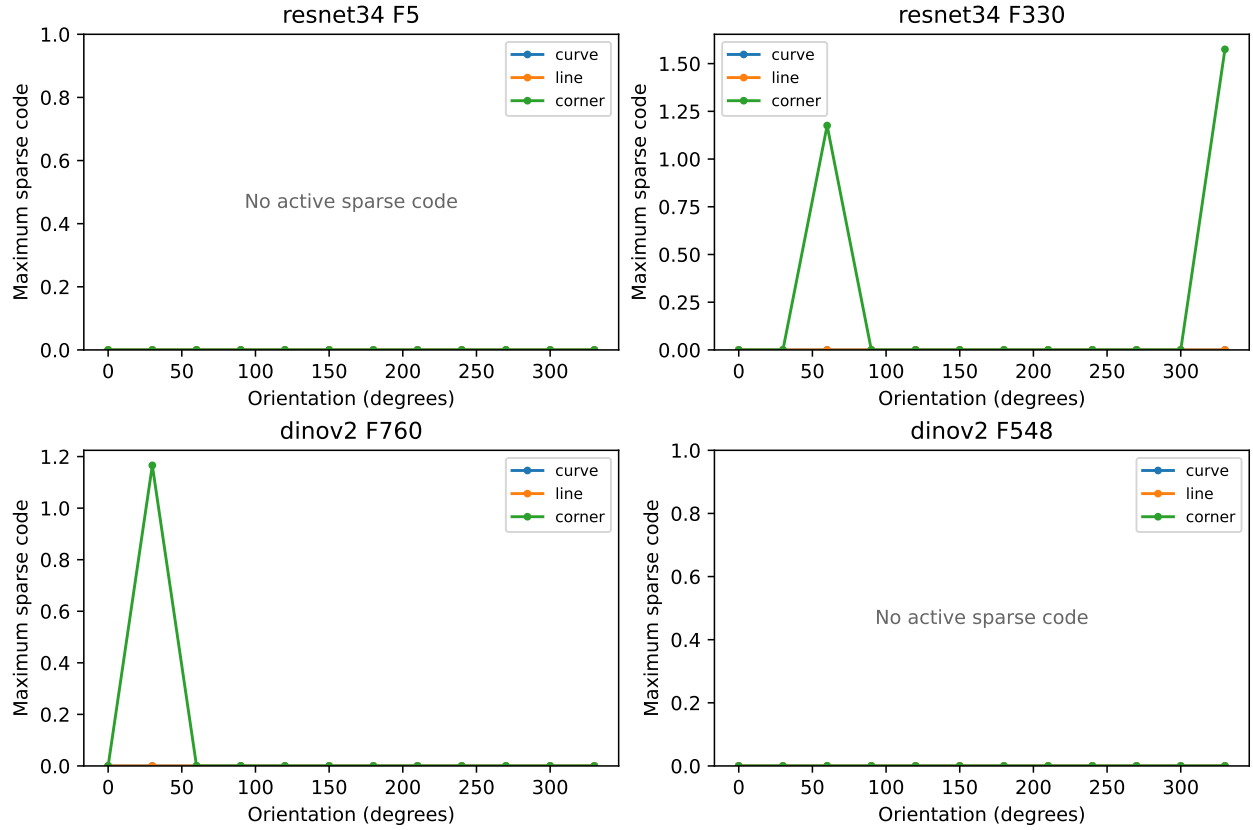
Figure 11: Actual sparse-coordinate responses to the controlled stimuli. Each panel reports one training-selected coordinate. A peak or a weak response here is an observation on this probe family, not a demonstration that the coordinate is a curve detector. Flat zero curves mean that Top- k gating suppresses that coordinate on these inputs.
