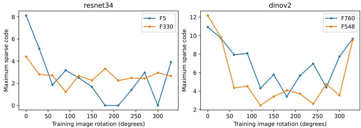
Figure 12: Responses under rotation of the fixed training references. Absolute code magnitudes are shown without rescaling each curve to its own maximum. Coordinates and backbones have different native units; compare transformations within a curve rather than absolute values across models.
