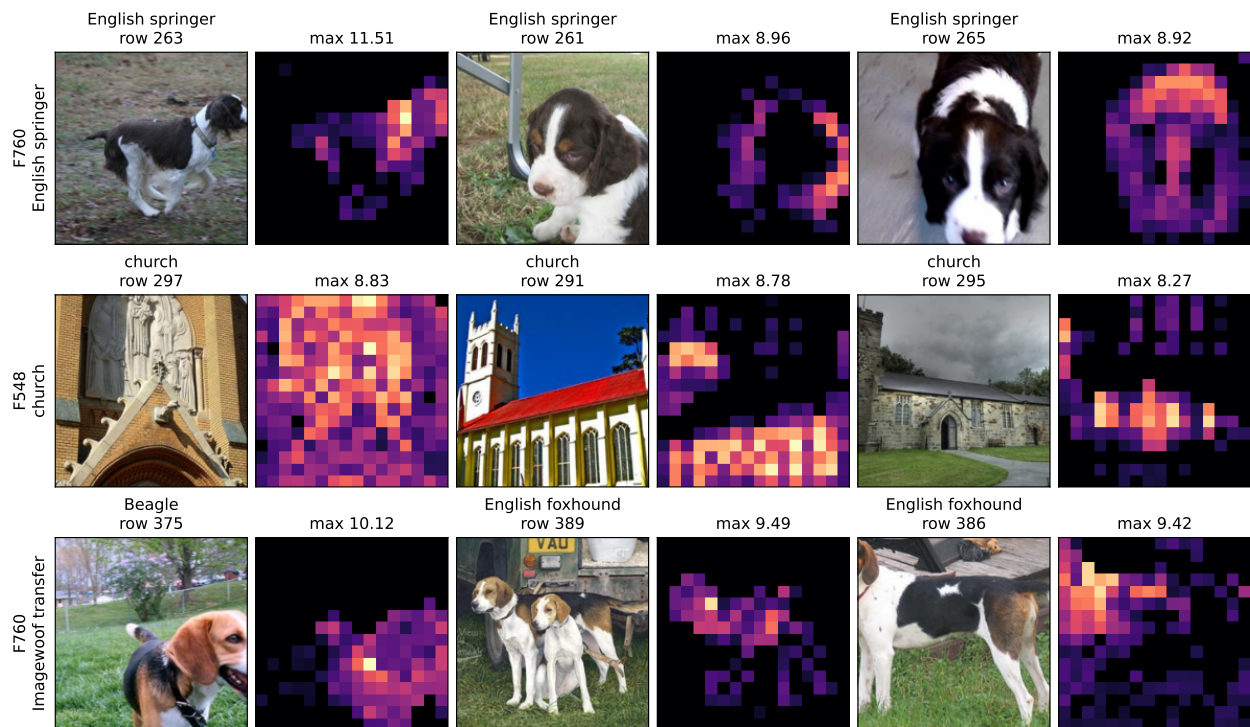
Figure 8: The same selection and evaluation protocol for DINOv2. Maps locate patch-token responses after global self-attention; they are not object masks. Imagenette and Imagewoof labels identify the photographs rather than certify the coordinate’s semantic meaning.
