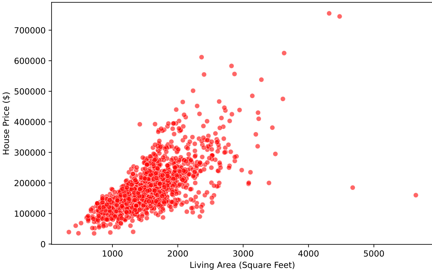
2. Living Area vs House Price (Outlier Detection)
