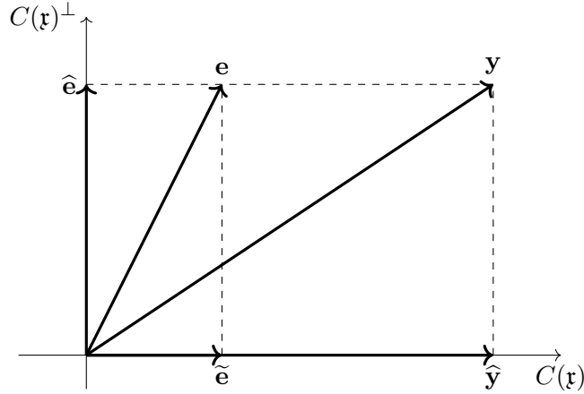
Figure 7.1: The geometry of the linear model
