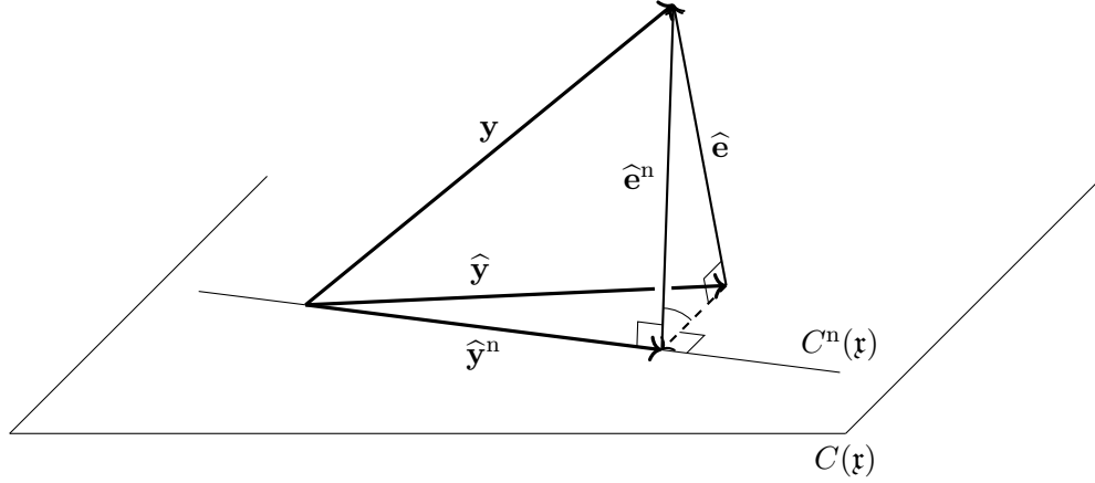
Figure 10.1: The geometry of nested models
