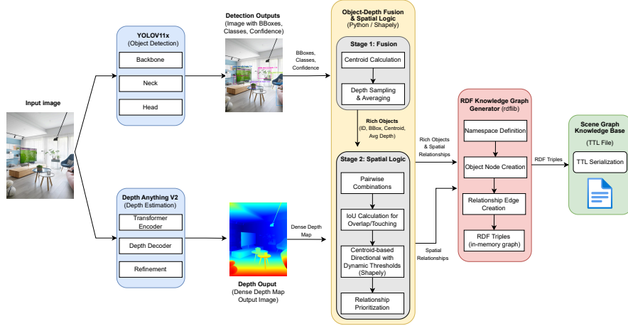
Fig. 1. Stage 1 architecture: Initial Visual-Spatial Knowledge Generation
