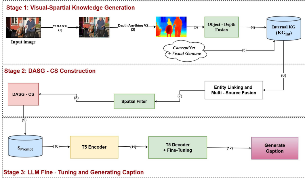
Fig. 1. Structure of proposed model for image captioning
