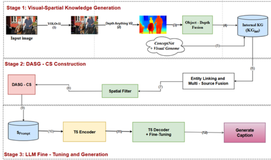
Fig. 1. Structure of proposed model for image captioning
