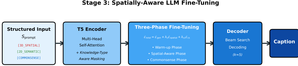
Fig. 4. Architecture of the Spatially-Aware LLM Fine-Tuning
