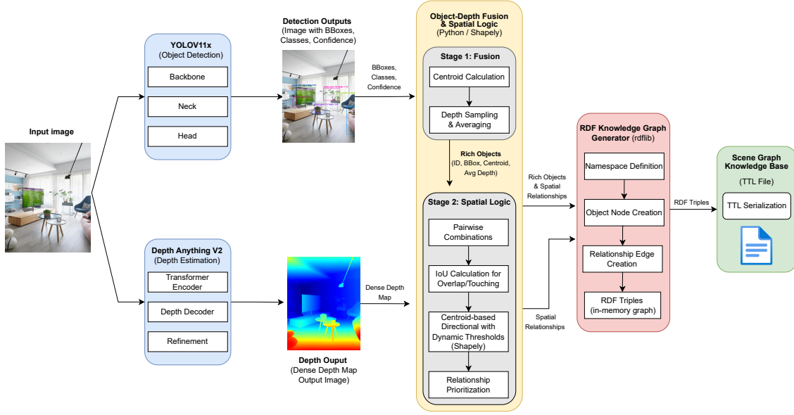
Fig. 2. An architecture of Initial Visual-Spatial Knowledge Generation
