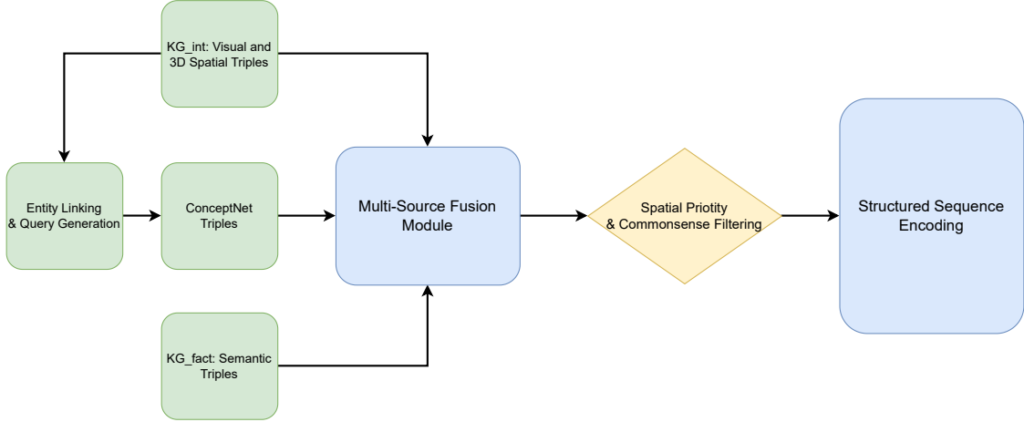
Fig. 3. Architecture of the DASG-CS Construction and Fusion Module
