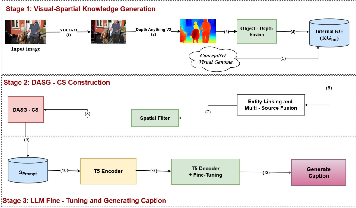
Fig. 1. Structure of proposed model for image captioning
