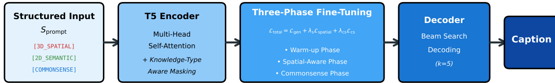
Fig. 4. Architecture of the Spatially-Aware LLM Fine-Tuning
