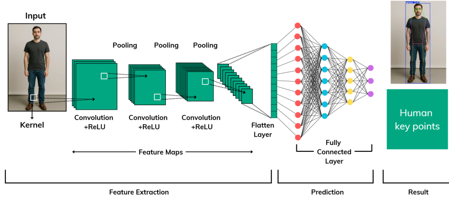
Fig. 1. Human Pose Detection Process
