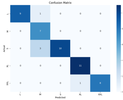
Fig. 3. Confusion matrix
