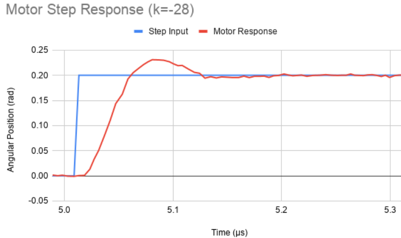
Figure 4: Motor response to step input when K_p = -28
