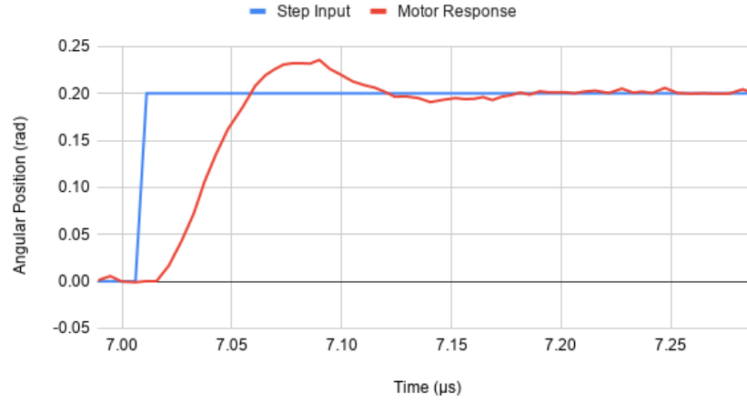
Motor Step Response (k=-30)
