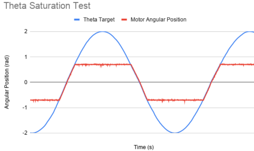
Figure 8: Theta Saturation Test
