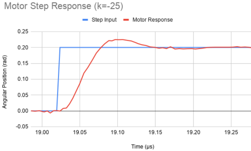
Figure 3: Motor response to step input when K_p = -25
