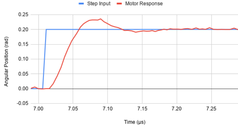
Motor Step Response (k=-30)
