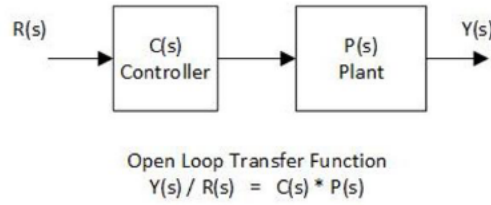
Figure 1: Open Loop System Block Diagram
