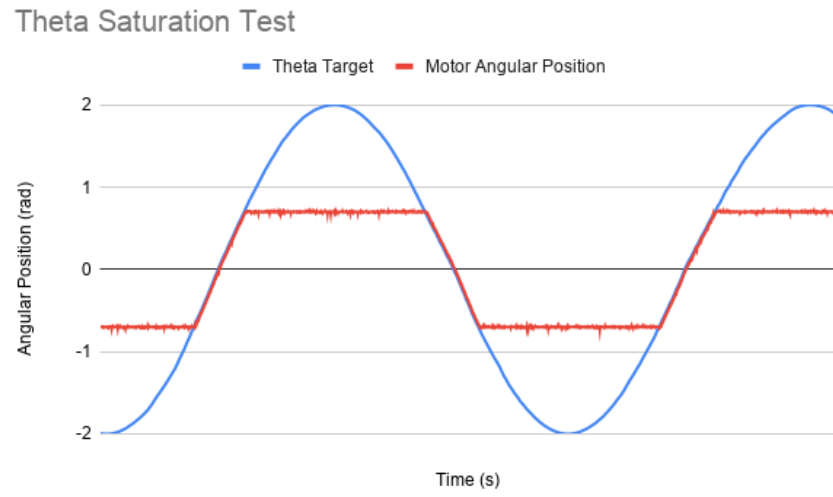
Figure 6: Theta Saturation Test
