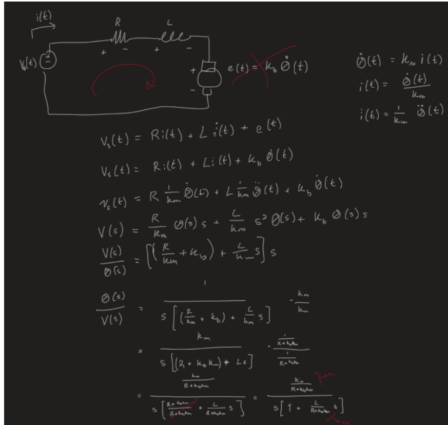
Figure 11: Standard DC Electric Motor Transfer Function Derivation
