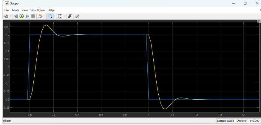
Figure 8: Closed-loop system model: step response
