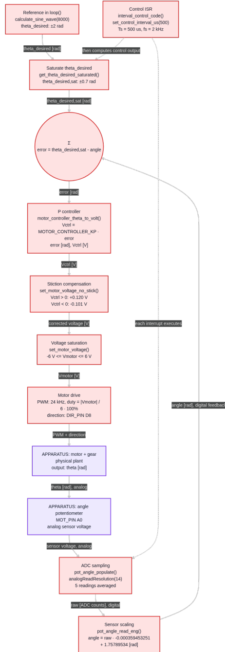
Figure 10: Inner-loop block diagram at the end of Lab 1.
