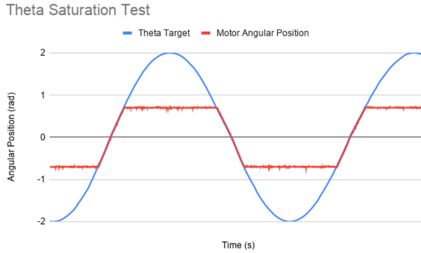
Figure 9: Theta Saturation Test
