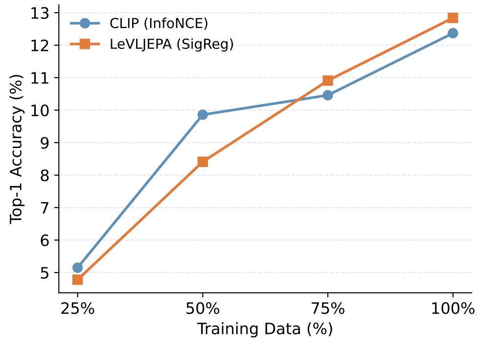
Zero-Shot Top-1
