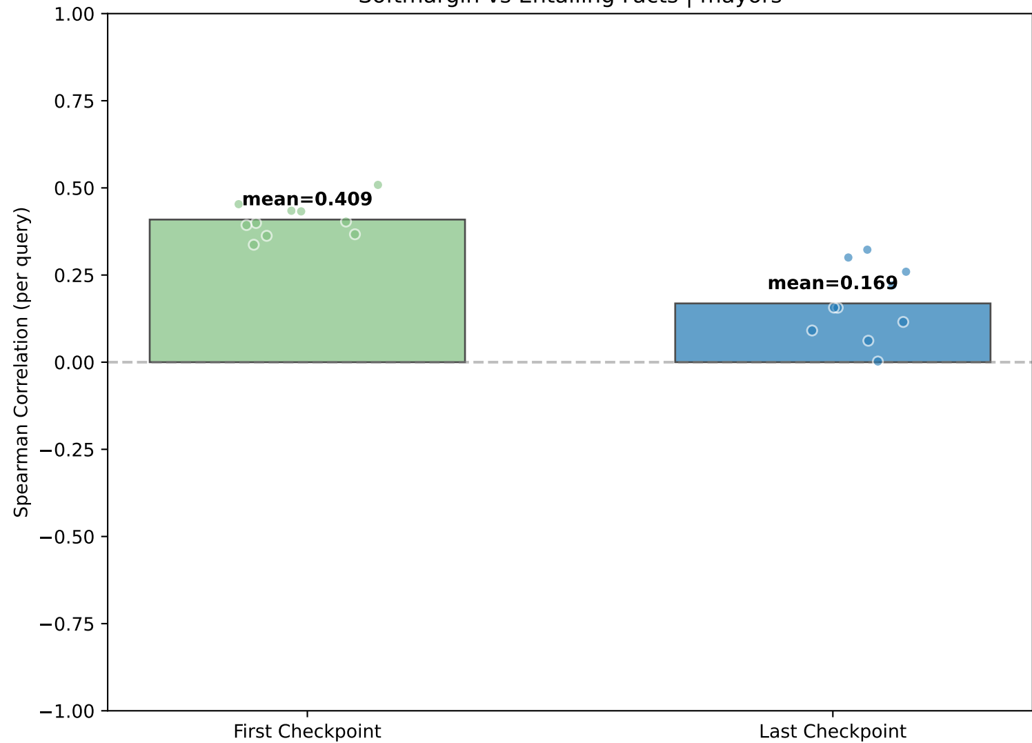
Softmargin vs Entailing Facts | mayors
