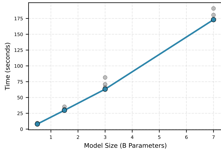
Fit Lambda
