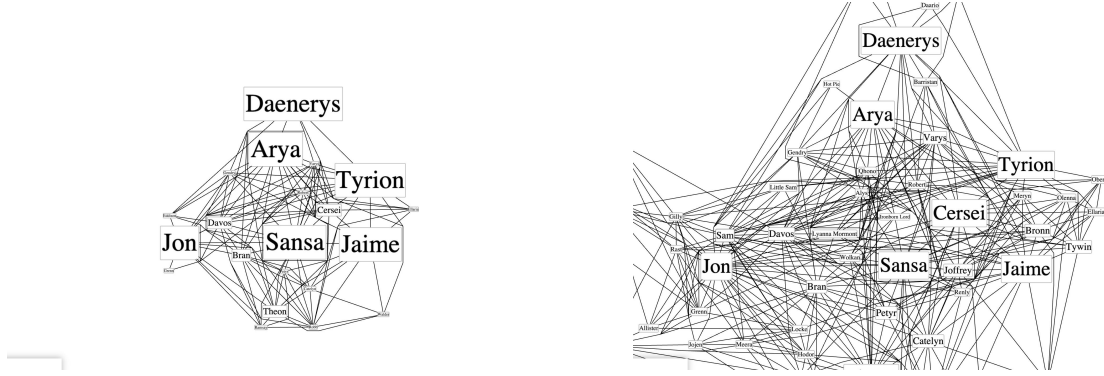
Figure 2: Two adjacent pyramid levels of the Game of Thrones graph rendered by the WebGL renderer of MSAGLJS with the sleeve router. The coarser level is on the left, the finer one on the right; both panels are cropped to the same world window. For each level a new graph is assembled from a PageRank-ranked prefix of the nodes, and edges are routed against the obstacles introduced at that level.
