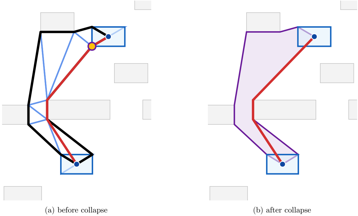
Figure 4: Effect of vertex collapse on the LORAS-RENNY edge of the Game of Thrones graph. Endpoints are shown as blue dots; their padded obstacles are highlighted in light blue. (a) The CDT triangles forming the sleeve are drawn in cornflower blue and the funnel path in red; the thick black polyline is the perimeter of the non-collapsed sleeve. The yellow dot marks the source-obstacle vertex that gets collapsed. (b) The sleeve after collapse, drawn as a single purple polygon with the source/target obstacles merged into the corresponding endpoints, and the funnel path (red) through it. Collapsing widens the funnel opening at the endpoint and removes the spurious detour around the obstacle corner.
