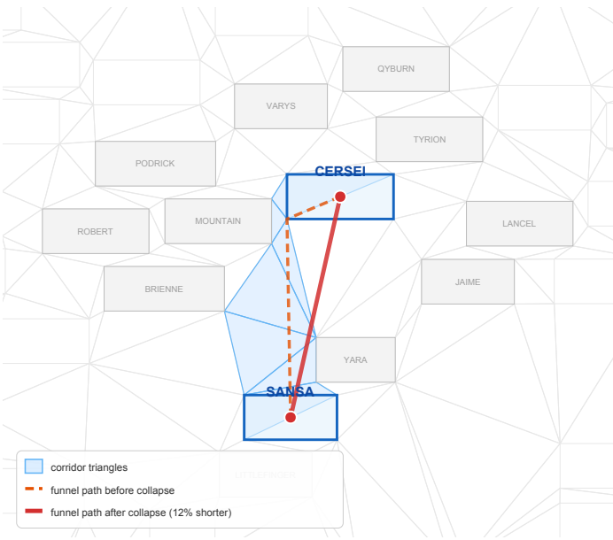
Figure 2 Effect of vertex collapse on the CERSEI–SANSA edge. Light blue: sleeve triangles. Orange dashed: funnel path before collapse (3 waypoints). Red solid: funnel path after collapse (2 waypoints, 12% shorter). Collapsing obstacle vertices to the node center widens the funnel opening and removes the detour.
