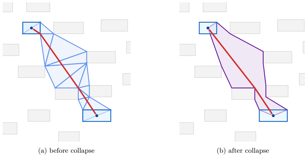
Figure 2 Effect of vertex collapse on the OSHA-SMALLJON edge of the Game of Thrones graph. Endpoints are shown as blue dots; their padded obstacles are highlighted in light blue. (a) The sleeve as a union of CDT triangles (light blue) and the funnel path through it (red, 7 waypoints). (b) The sleeve after collapse, drawn as a single purple polygon with the source/target obstacles merged into the corresponding endpoints, and the funnel path through the collapsed sleeve (red, 5 waypoints, 21% shorter). Collapsing widens the funnel opening at each endpoint and removes the spurious detours around obstacle corners.
