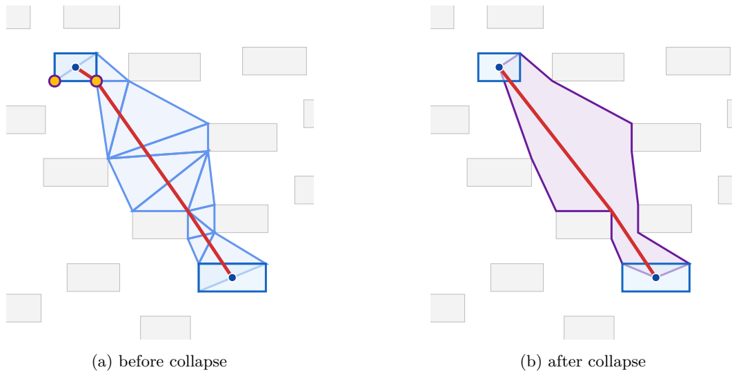
330 Figure 2 Effect of vertex collapse on the OSHA-SMALLJON edge of the Game of Thrones graph. 331 Endpoints are shown as blue dots; their padded obstacles are highlighted in light blue. (a) The 332 sleeve as a union of CDT triangles (light blue) and the funnel path through it (red, 7 waypoints). 333 The two yellow dots mark the source-obstacle vertices that get collapsed, one on each chain. (b) The 334 sleeve after collapse, drawn as a single purple polygon with the source/target obstacles merged into 335 the corresponding endpoints, and the funnel path through the collapsed sleeve (red, 5 waypoints, 336 21% shorter). Collapsing widens the funnel opening at each endpoint and removes the spurious 337 detours around obstacle corners.
